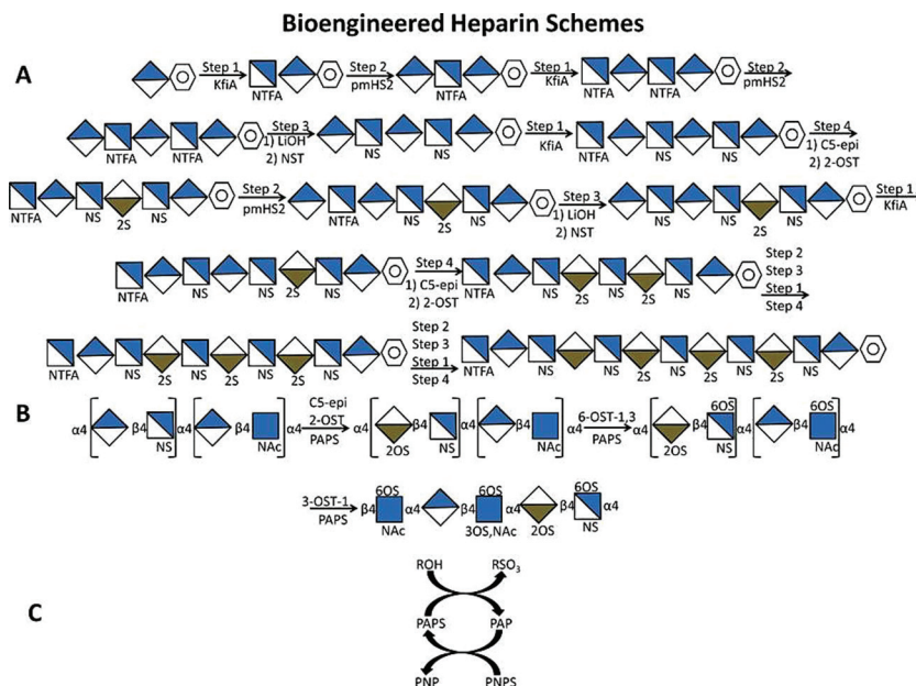
Figure 6. Chemoenzymatic synthesis of heparin. A) Homogenous low molecular weight heparin scheme. B) Enzymatic portion of the bioengineered heparin scheme. C) Cofactor recycling where 3'-phosphoadenosine-5'-phosphosulfate (PAPS) is generated from 3'-phosphoadenosine-5'-phosphate (PAP) using aryl sulfotransferase IV and p -nitrophenol sulfate (PNPS) as a sacrificial sulfo group donor affording p -nitrophenol (PNP). The symbols used are defined in Figure 5.
