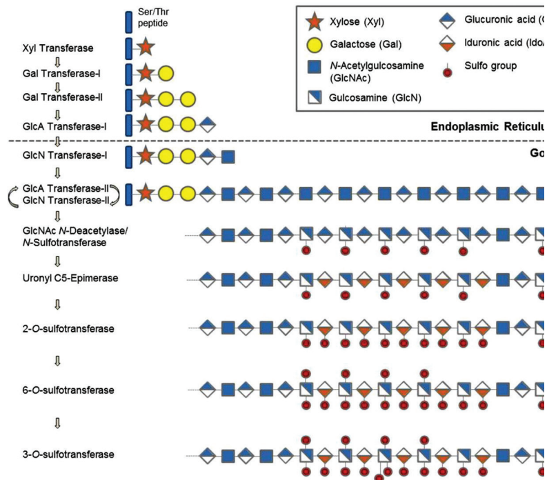
Figure 5. Biosynthetic pathway of heparin and heparan sulfate proteoglycan (HSPG). The glycosaminoglycan-protein linkage region is assembled by several glycosyltransferases. Repeating disaccharide unit is then elongated by GlcA and GlcN transferases. Next, various modifications, such as N-deacetylation and N-sulfonation of glucosamine, conversion of GlcA to IdoA, and O-sulfonations, take place through the actions of the specific enzymes shown.
