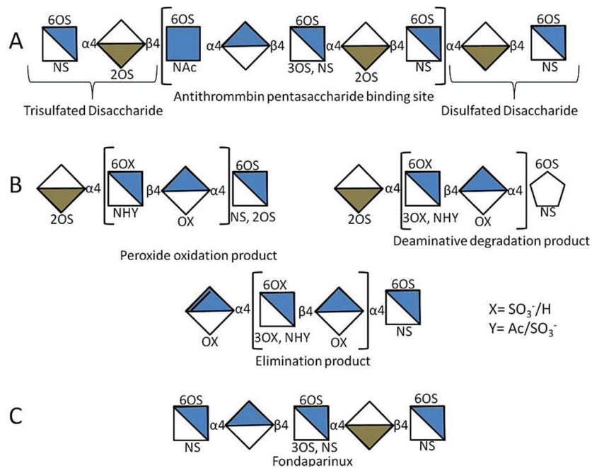
Figure 4. Structure of unfractionated heparin (UFH), low molecular weight heparin (LMWH) and ultra low molecular weight heparin (ULMWH). The brackets shown indicate multiple copies of the domains. A) Major domains in UFH are labeled. There are typically a combined number of 20 to 50 copies of both trisulfated and disulfated domains in UFH. B) LMWHs synthesized using different methods. Three major methods and typical structures with reducing and non-reducing ends are shown. Approximately 7-10 of the domains, shown in brackets, are present in each LMWH. C) AT binding domain of the ULMWH, fondaparinux. The symbols used are defined in Figure 5.
