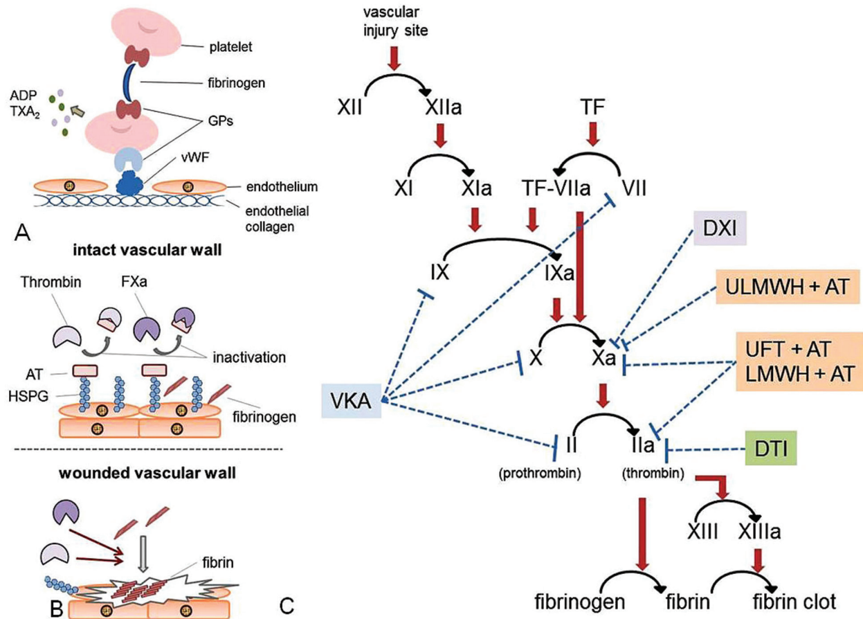
Figure 1. Coagulation pathway. A) Molecular mechanism of a platelet adhesion and aggregation involving von Willibrand factor (vWF) and glycoproteins (GPs), releasing adenosine diphosphate (ADP) and thromboxane A2 (TXA 2 ). B) Endothelial heparan sulfate proteoglycan (HSPG) interaction with antithrombin (AT) resulting in the inactivation of thrombin and factor Xa (FXa) to control coagulation. C) Main reactions of the coagulation cascade after activation through vascular injury or by tissue factor (TF) and major clinical anticoagulants including direct factor Xa inhibitor (DXI), direct thrombin inhibitor (DTI) and vitamin K antagonists (VKAs).
