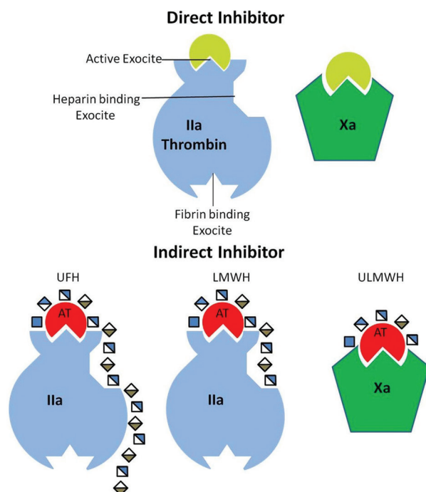
Figure 2. Schematic representation of direct inhibitors, including direct thrombin (FIIa) inhibitors (DTIs), Direct factor Xa inhibitors (DXIs) and indirect inhibitors, antithrombin (AT) with unfractionated heparin (UFH), low molecular weight heparin (LMWH) and ultra low molecular weight heparin (ULMWH), of factor IIa and factor Xa. The heparin sequence displayed in this figure corresponds to the pentasaccharide binding site (containing N -acetylglucosamine, glucuronic acid, glucosamine, idouronic acid, and glucosamine residues, respectively) and repeating idouronic acid, and glucosamine residues. Sulfo groups are not shown for simplicity. The symbols used are defined in Figure 5.
